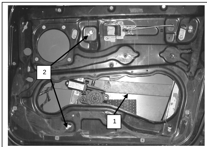
Porta lato destro, Portière avant droite, Right front door, Puerta lado derecho, Vorne rechte Tür, Porta frente dirieta, Sag on kapı, πόρτα εμπρόςδεξιά
